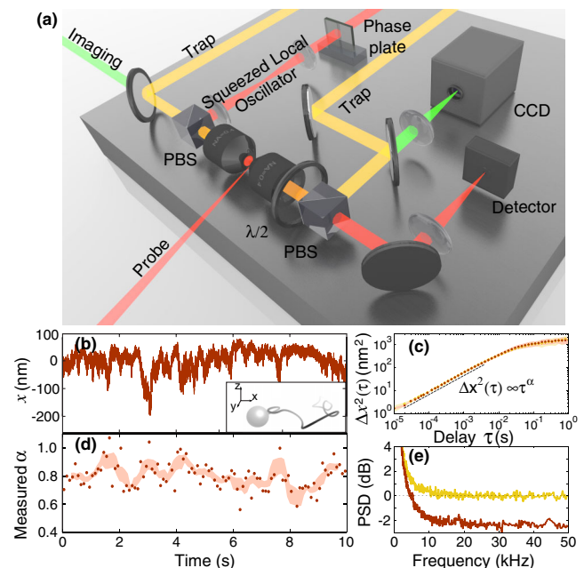
FIG. 1 (color online). Experimental setup. (a) Counterpropagating trapping fields (orange) confine particles between two objectives and are isolated from the detector with polarizing beam splitters (PBS) and wave plates ( \lambda/2 ). An imaging field (green) allows visual identification of the particles near the optical trap on a CCD camera. The particle tracking measurement relies only on an amplitude-squeezed local oscillator and an amplitude-modulated probe (red), with the probe providing dark-field illumination, and the particle tracking signal arising from interference between scattered light from the probe and the local oscillator. (b) Measured particle motion, which is the x projection of the 3D motion (shown schematically in the inset). (c) The MSD is constructed with both squeezed light (dark red) and coherent light (gold), and \alpha is determined by fitting this to Eq. (2). The classical and squeezed example traces here both yield \alpha = 0.83 . (d) The raw data are divided into 100 ms segments and the value of \alpha established for each (solid dots). The light red shaded region represents the moving mean and standard error with a 0.5-s width. (e) The normalized power spectral density (PSD) shows that squeezing suppresses the noise floor by 2.4 dB.
